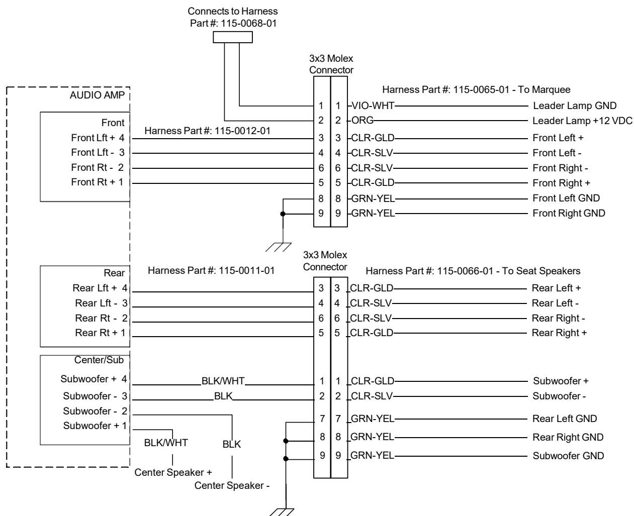
Figure 57. Audio Wiring
